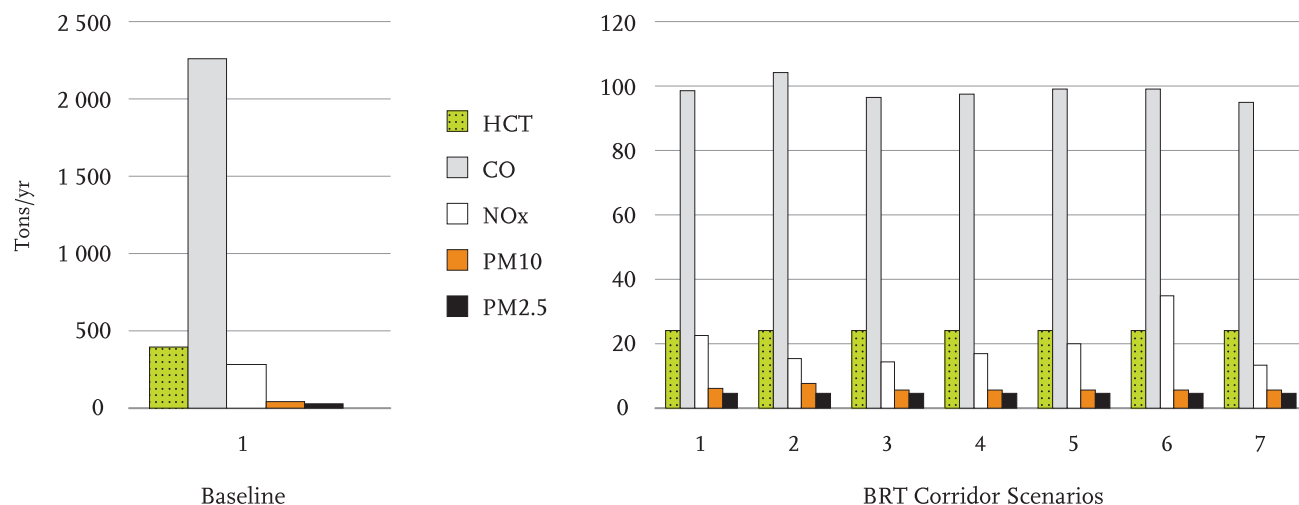
FIGURE 12 | CRITERIA POLLUTANT EMISSIONS FROM BASELINE AND BRT SCENARIOS
