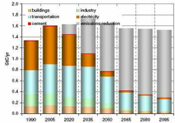
CO2 Emissions by Sector
