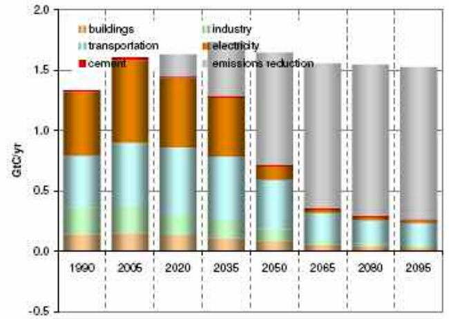
CO2 Emissions by Sector
