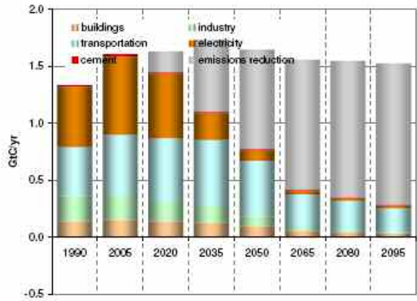
CO2 Emissions by Sector
