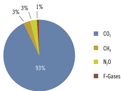
Figure 4.6 | Indiana GHG Emissions by Gas: 2003
